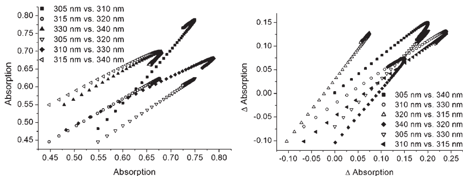
Figure 7. (a) Extinctions plot. (b) Differential extinctions plot.
