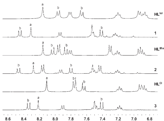
Figure 1. 1 H NMR spectra (aromatic region in DMSO- d 6 ) of HL tol , [ReOCl 2 (L tol )] (1), HL tBu , [ReOCl 2 (L tBu )] (2), HL Cl , and [ReOCl 2 (L Cl )] (3): (a) imino proton resonance, (b) pyridazine resonances, other resonances can be assigned to the protons of the phenolate ring.
