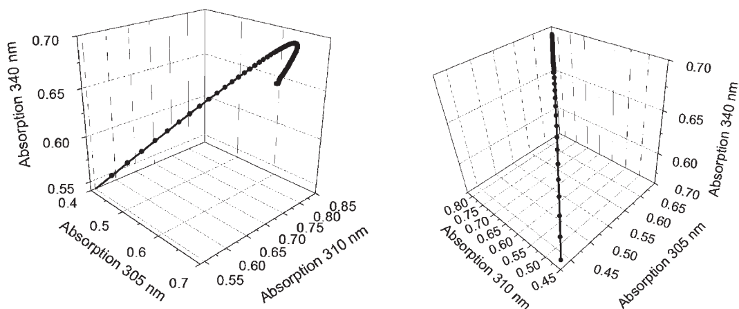
Figure 9. (a) Three-dimensional absorption–absorption–absorption correlations and (b) projection.
