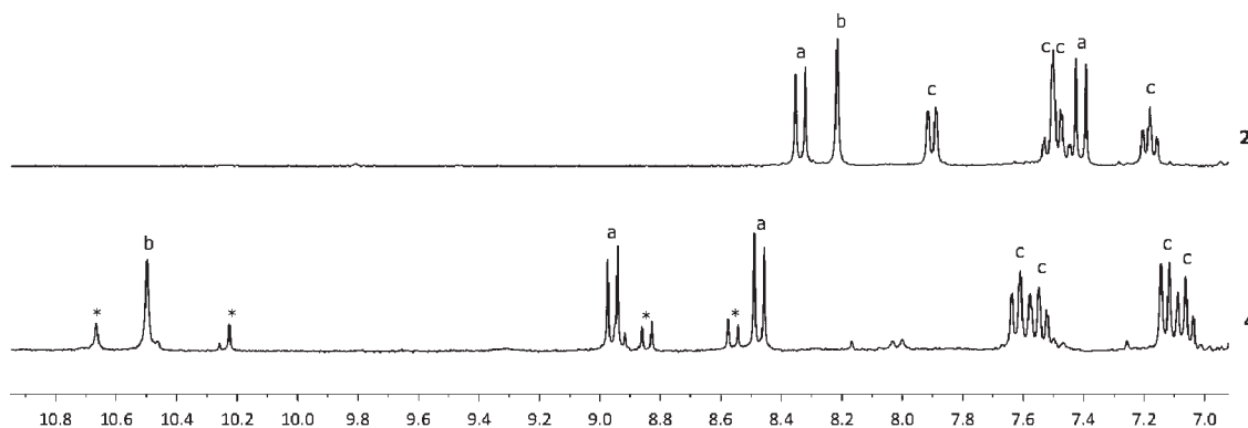
Figure 5. ^1\text{H} NMR spectra (aromatic region in \text{DMSO-}d_6 ) of [\text{ReOCl}_2(\text{L}^{\text{Bu}})] (2) and the crude product (4) obtained after reaction with 10 equiv of TBHP after 8 h: (a) pyridazine resonances, (b) imino signal, (c) aromatic phenolate signals. Asterisks (*) marked unidentified impurities.
