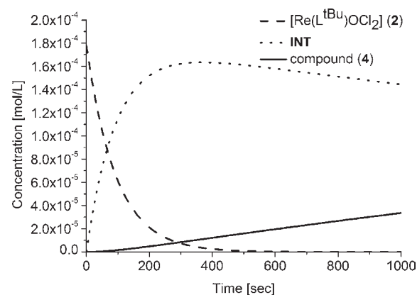
Figure 12. Species distribution curves of compounds 2, INT, and 4.
